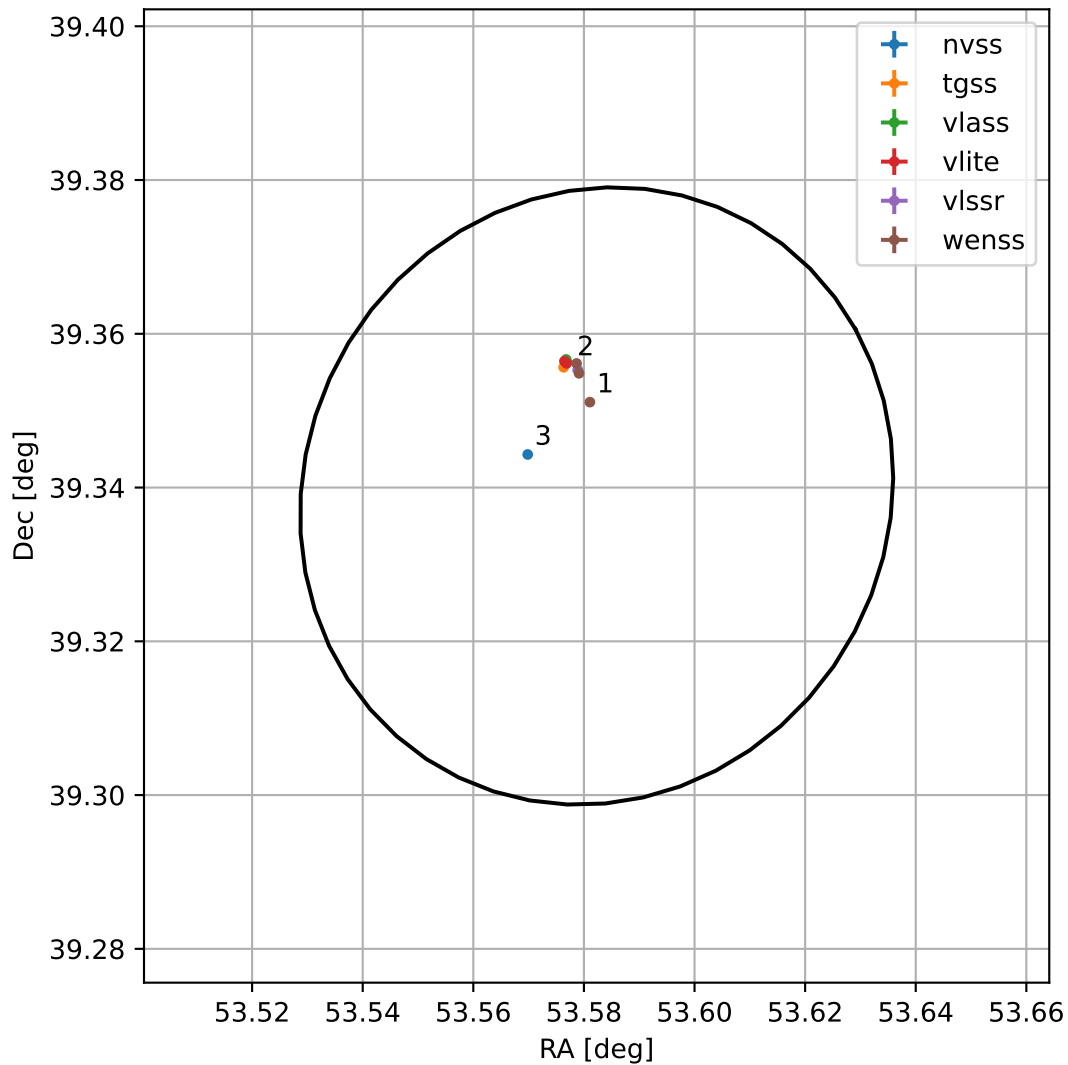
4FGL J0334.3+3920
