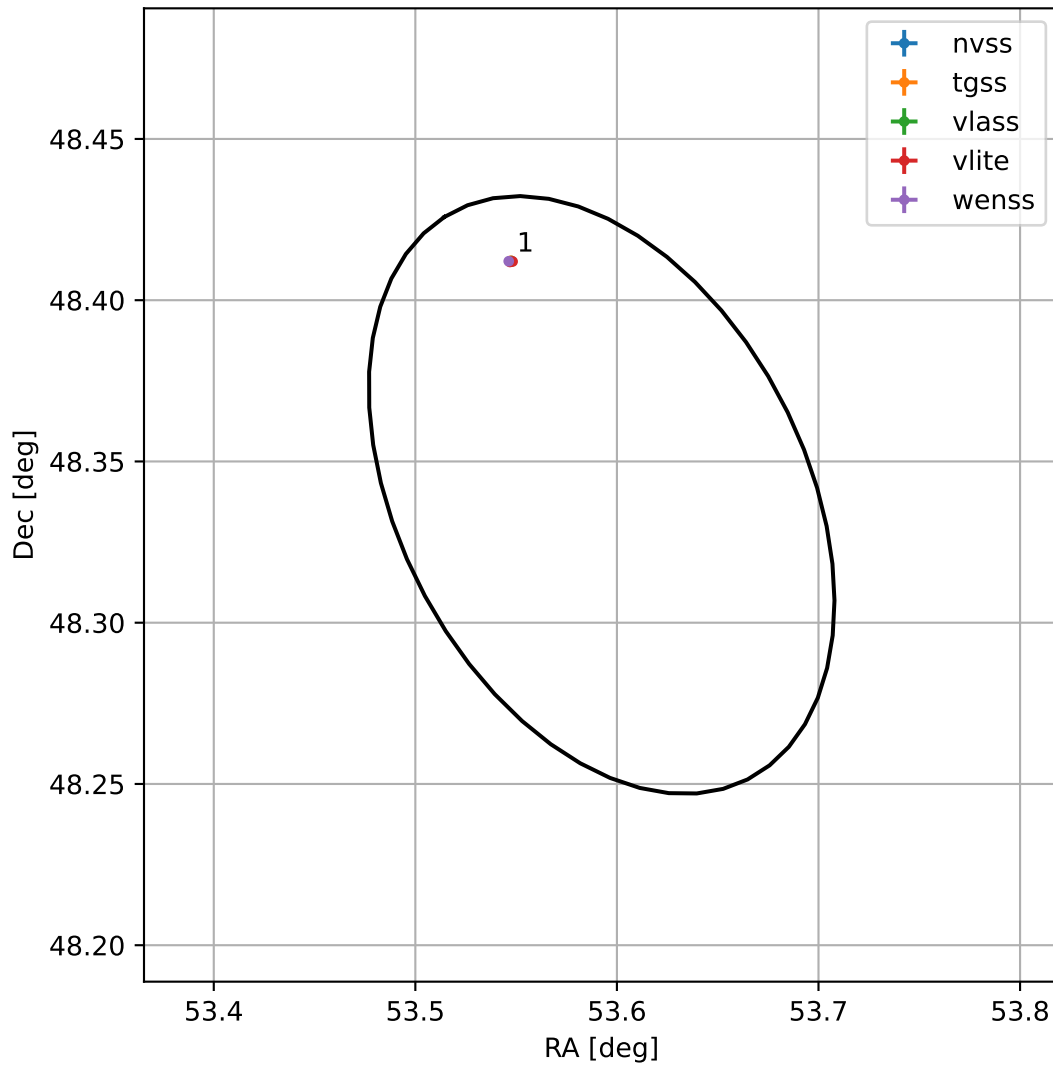
4FGL J0334.3+4820
