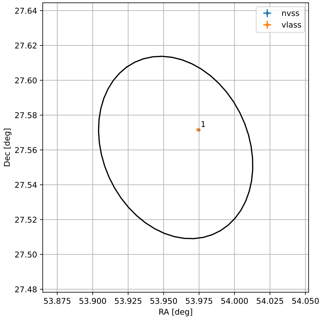
4FGL J0335.8+2733
