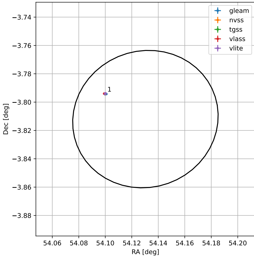
4FGL J0336.5-0348
