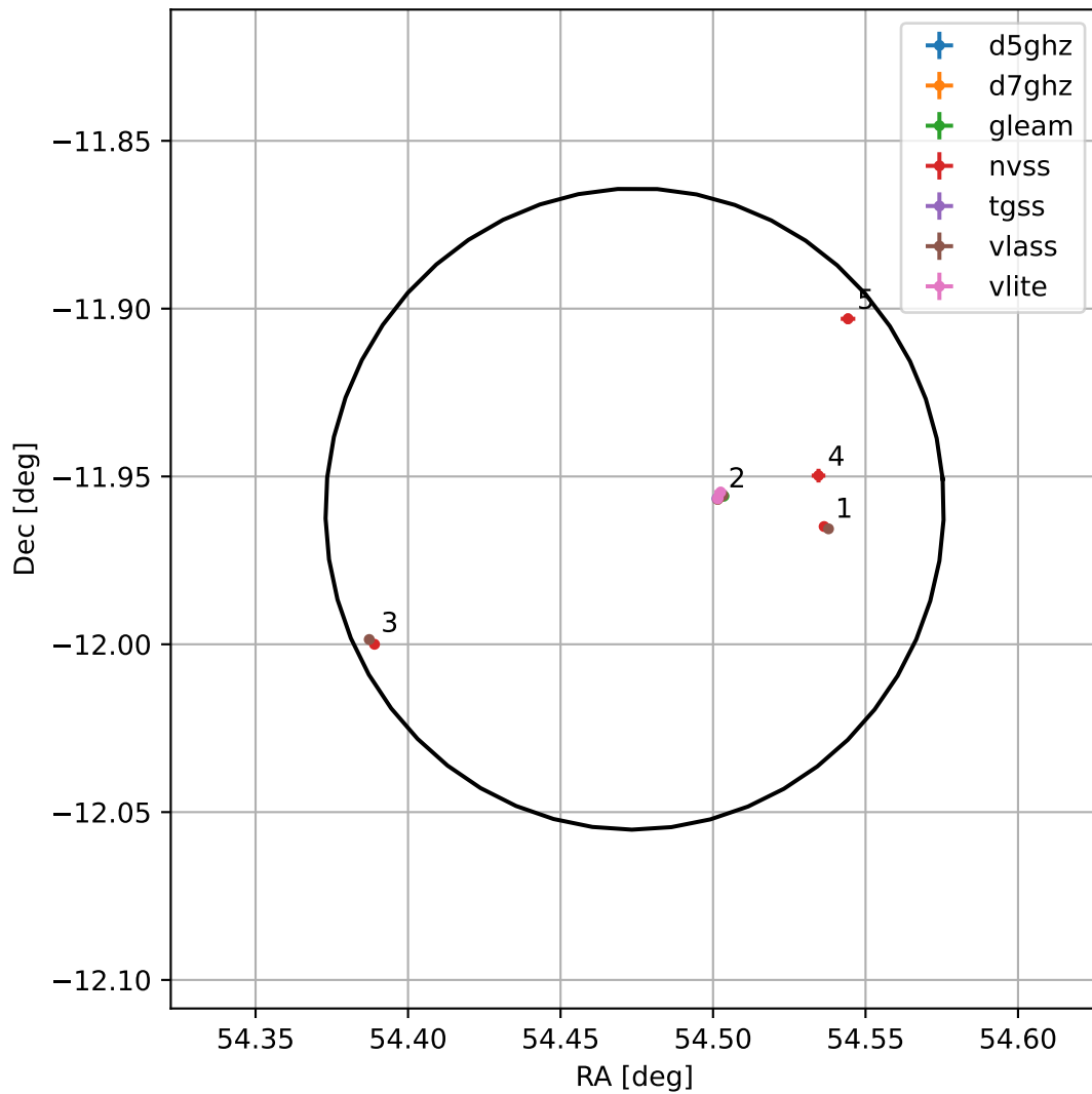
4FGL J0337.8-1157
