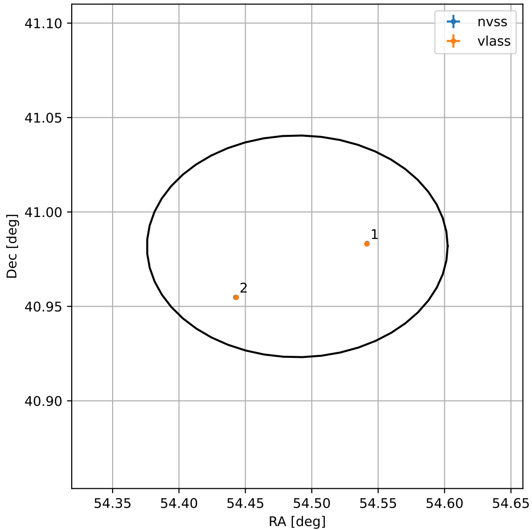
4FGL J0337.9+4058
