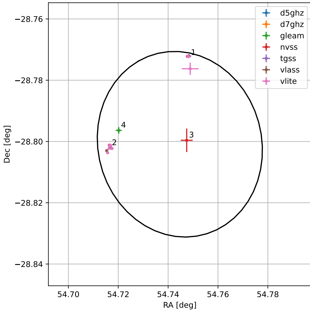
4FGL J0338.9-2848
