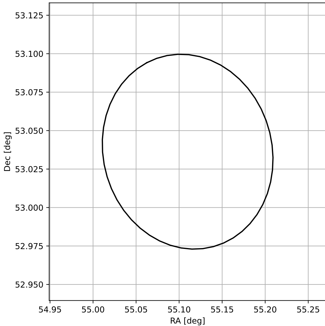
4FGL J0340.4+5302
