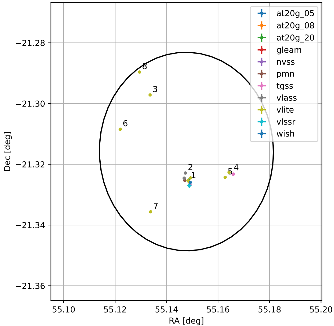
4FGL J0340.5-2118
