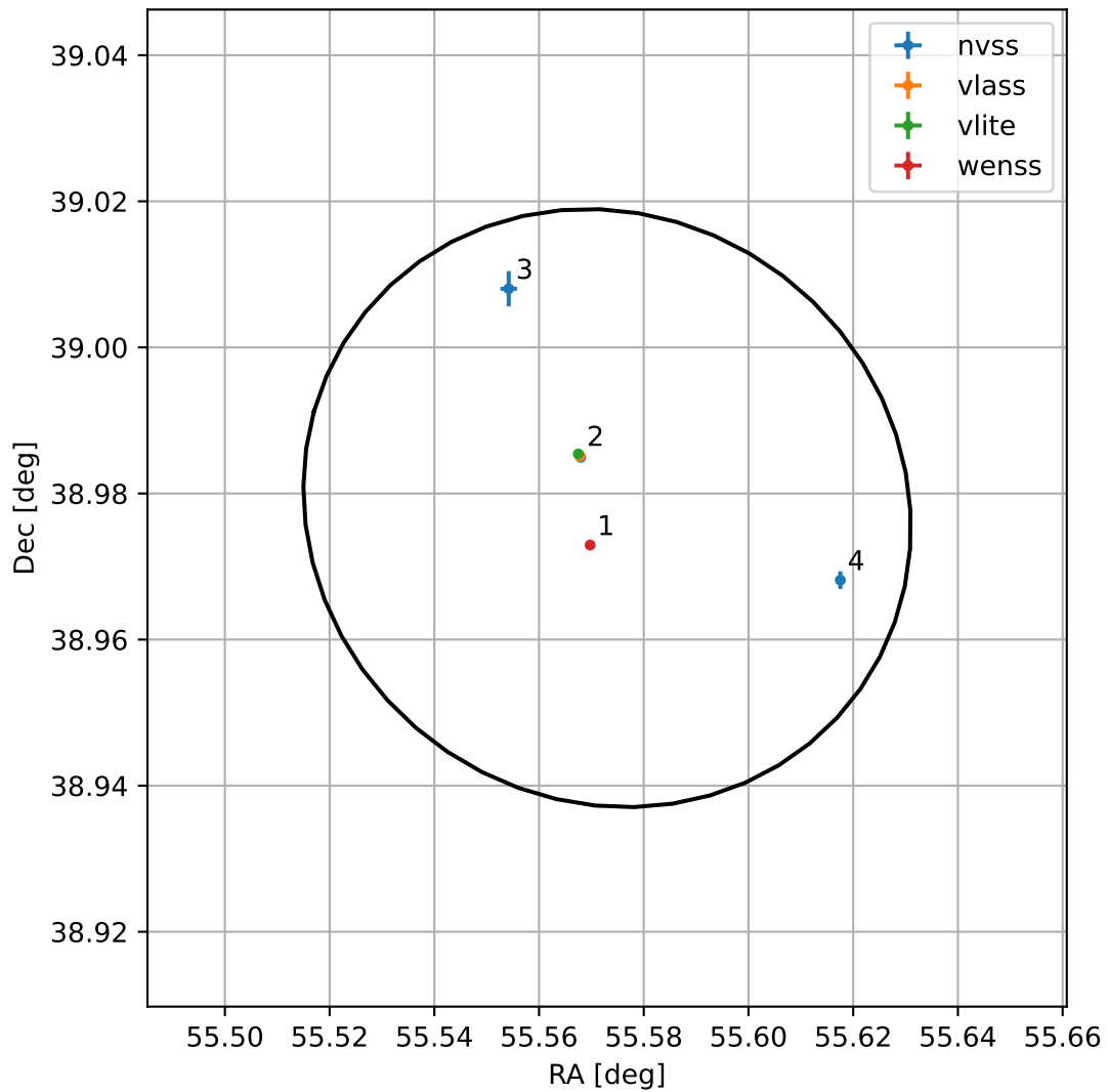
4FGL J0342.2+3858
