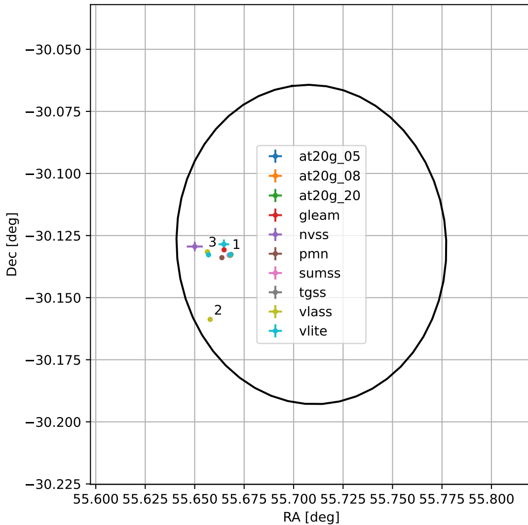
4FGL J0342.8-3007
