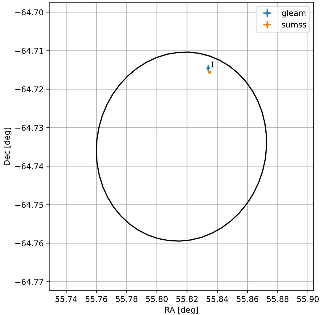
4FGL J0343.2-6444
