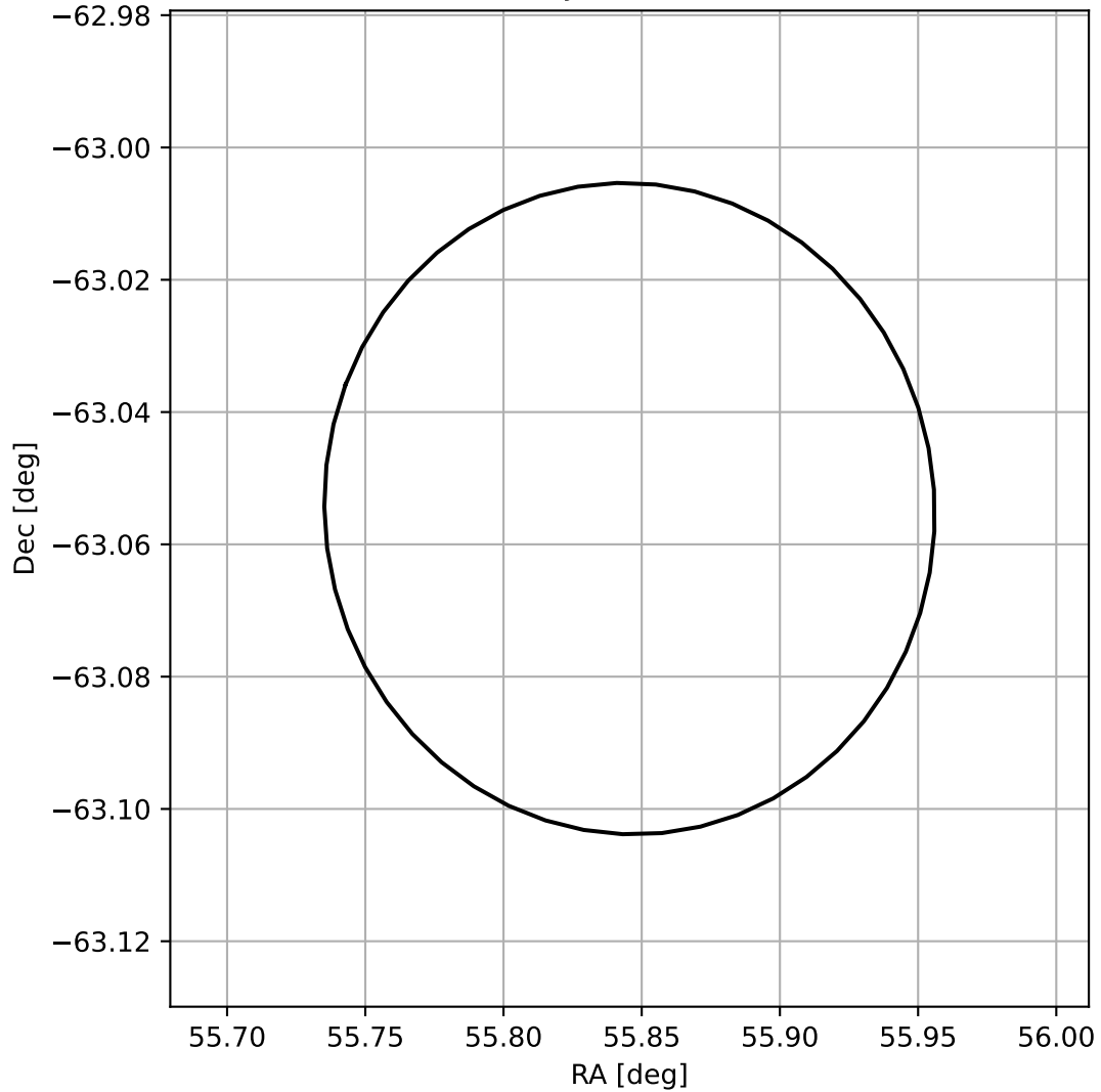
4FGL J0343.3-6303
