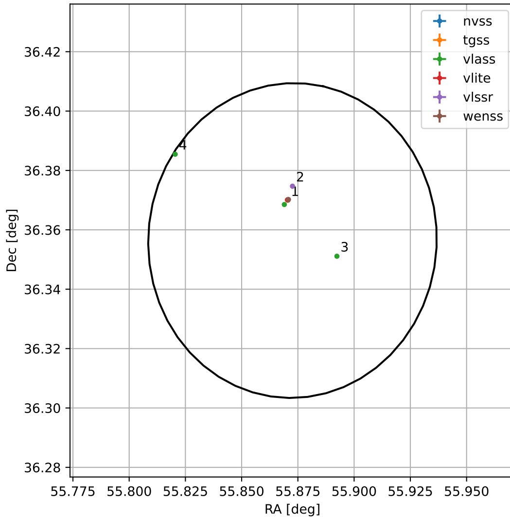
4FGL J0343.4+3621
