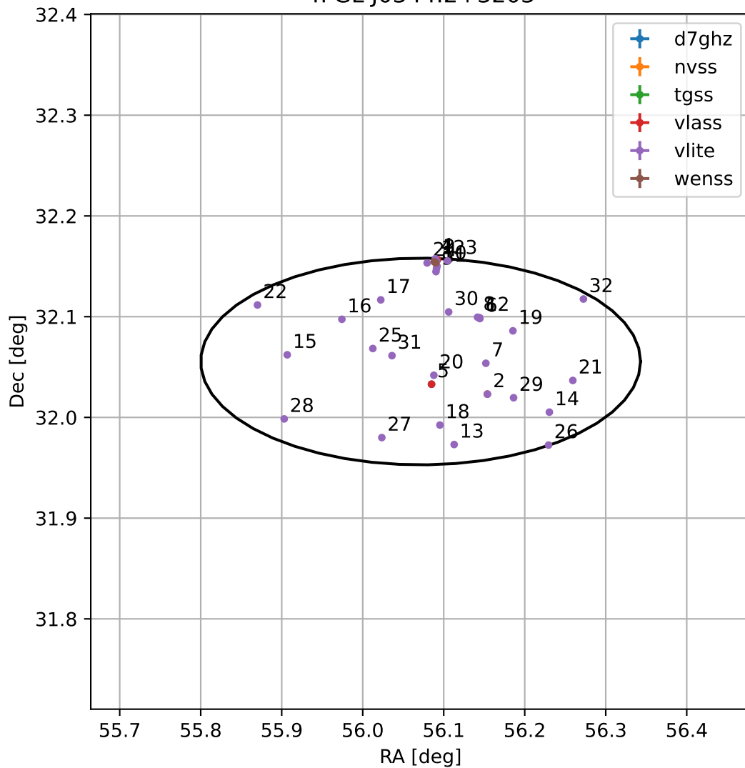
4FGL J0344.2+3203
