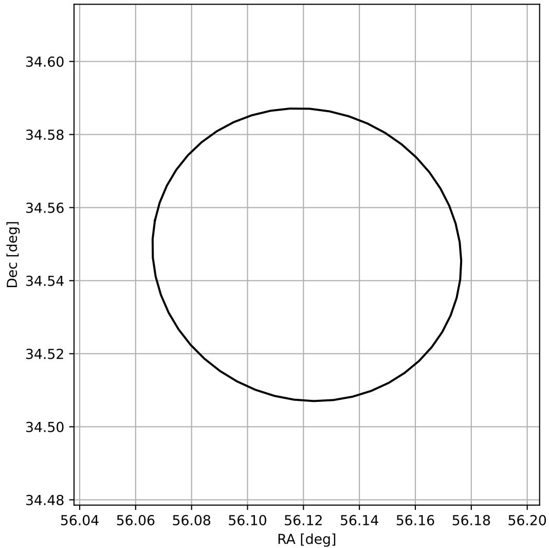
4FGL J0344.4+3432
