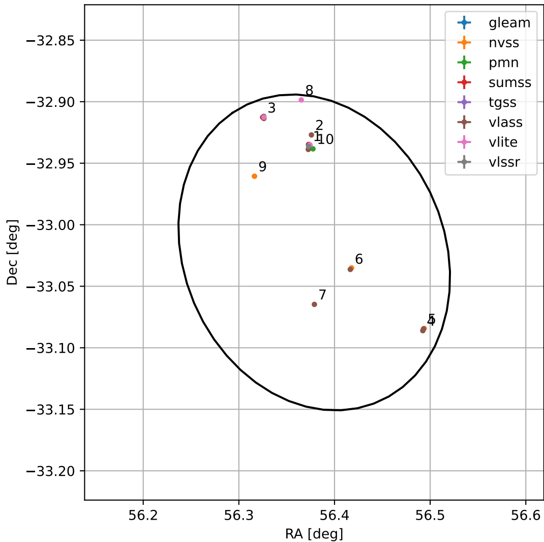
4FGL J0345.5-3301
