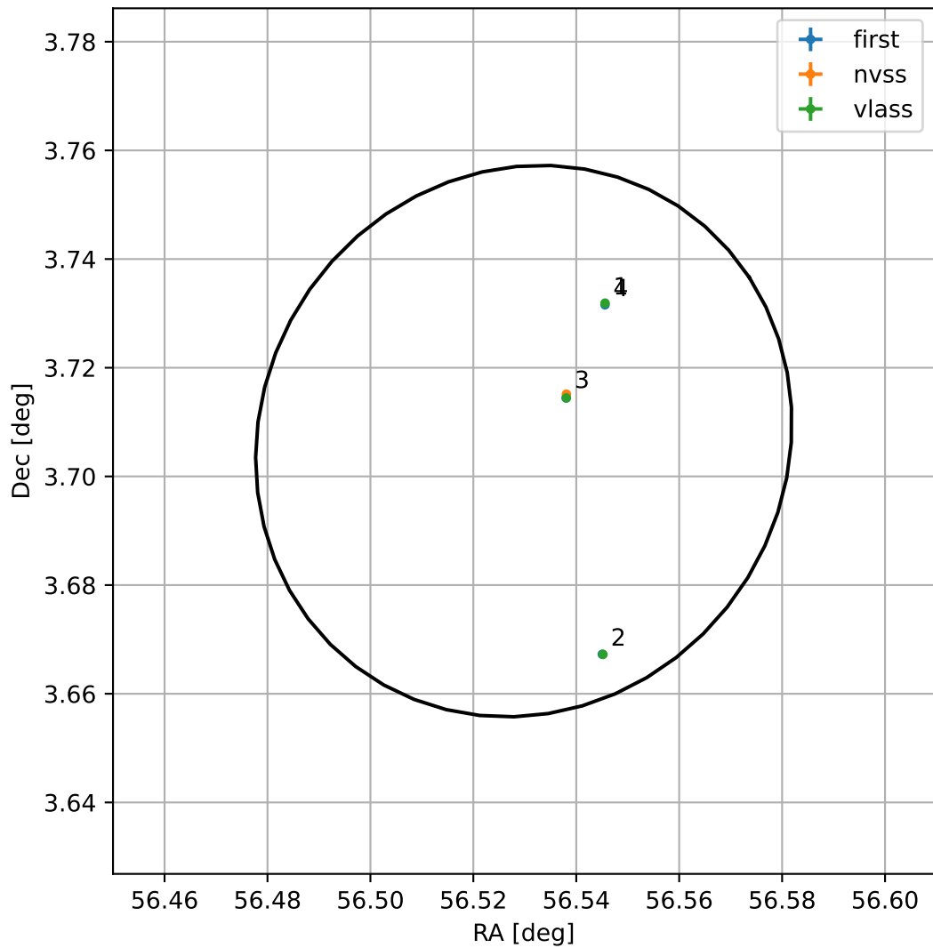
4FGL J0346.1+0342
