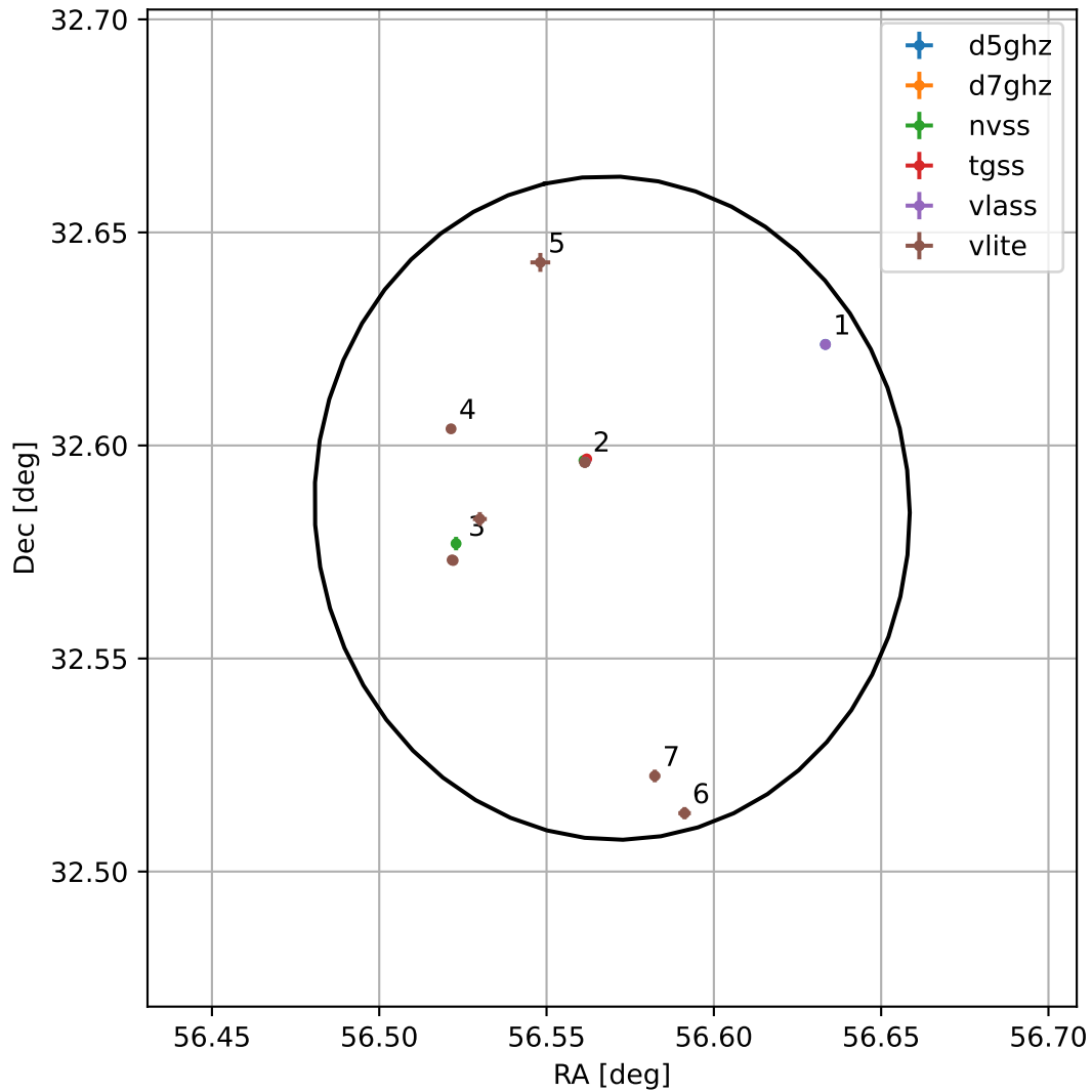
4FGL J0346.2+3235
