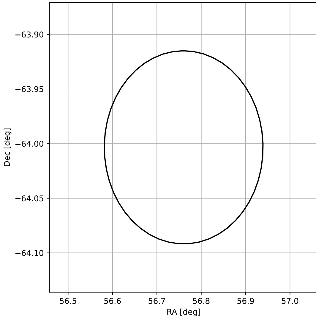
4FGL J0347.0-6400
