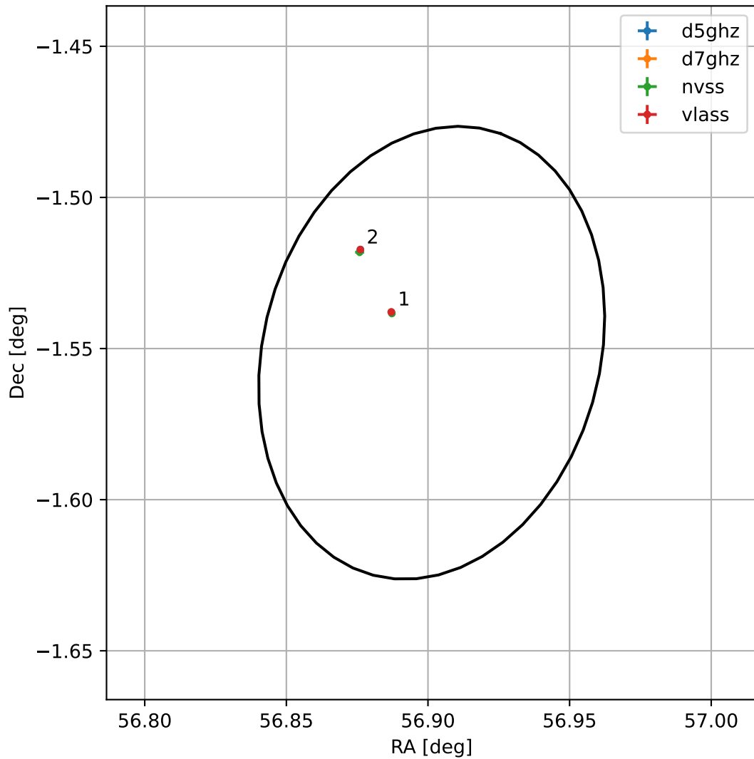
4FGL J0347.6-0133
