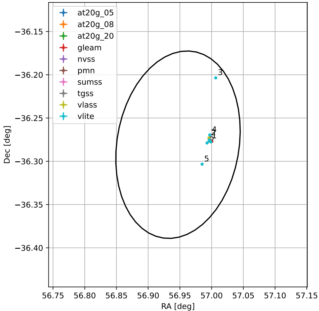
4FGL J0347.7-3616
