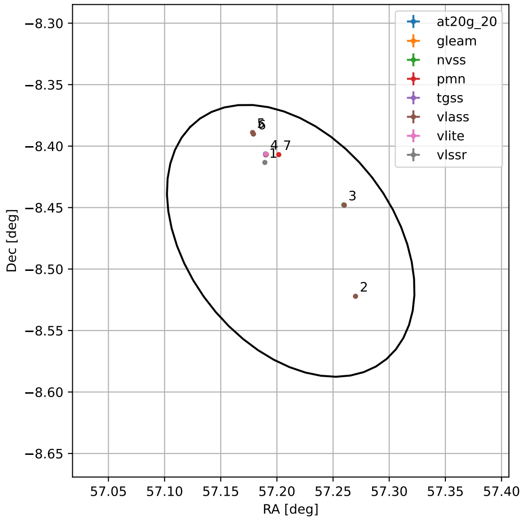
4FGL J0348.8-0828
