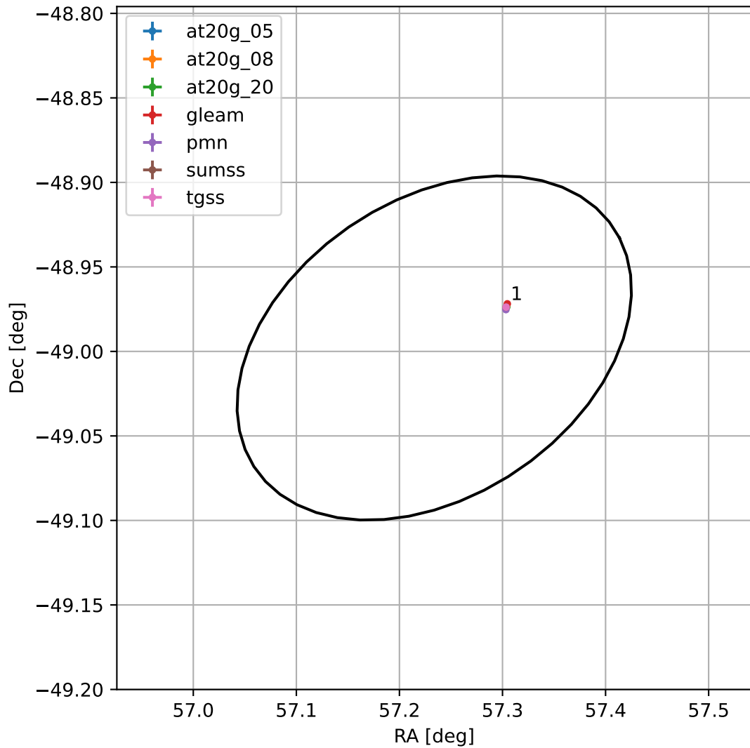
4FGL J0348.9-4859
