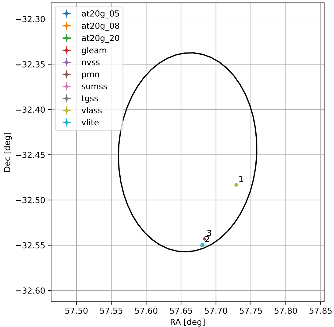
4FGL J0350.6-3226
