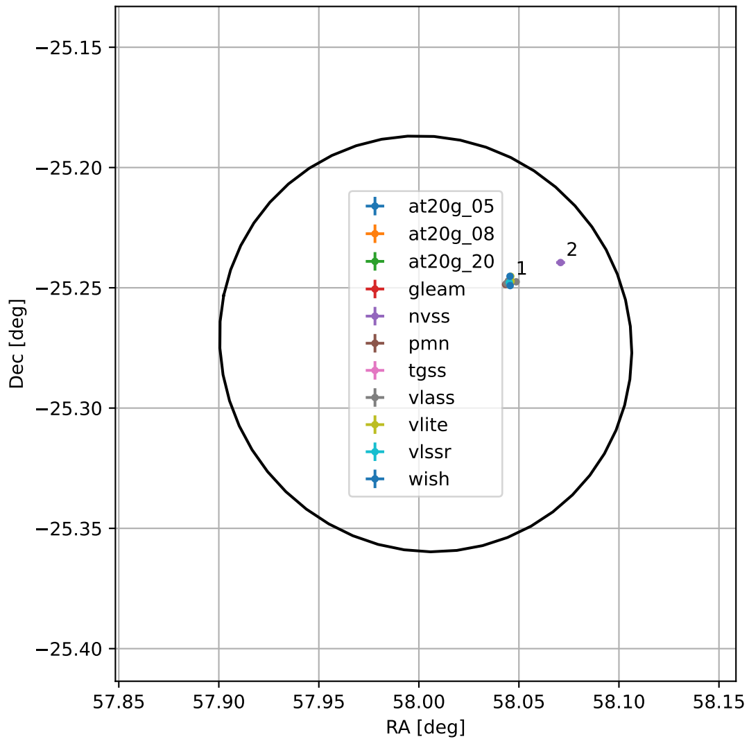
4FGL J0352.0-2516
