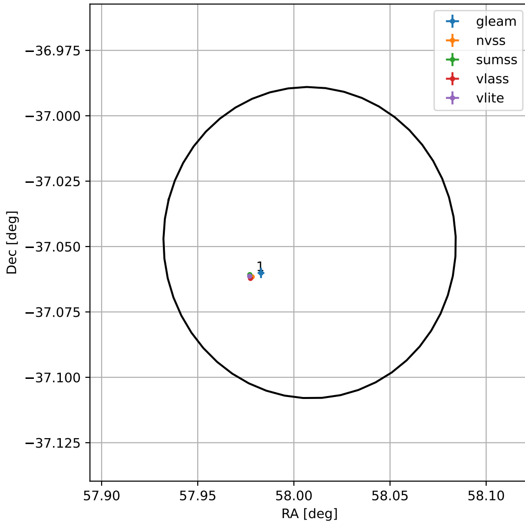
4FGL J0352.0-3702
