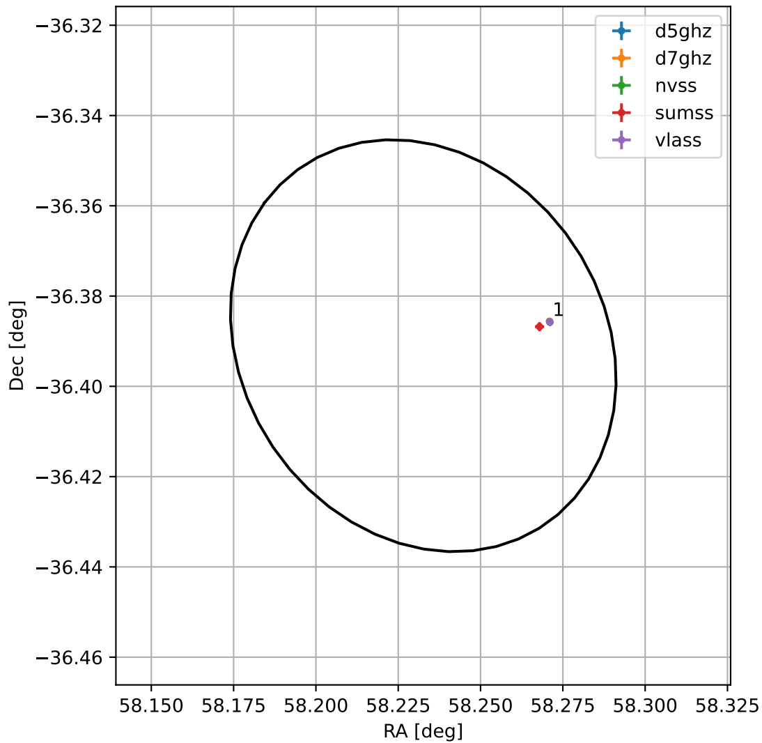
4FGL J0352.9-3623
