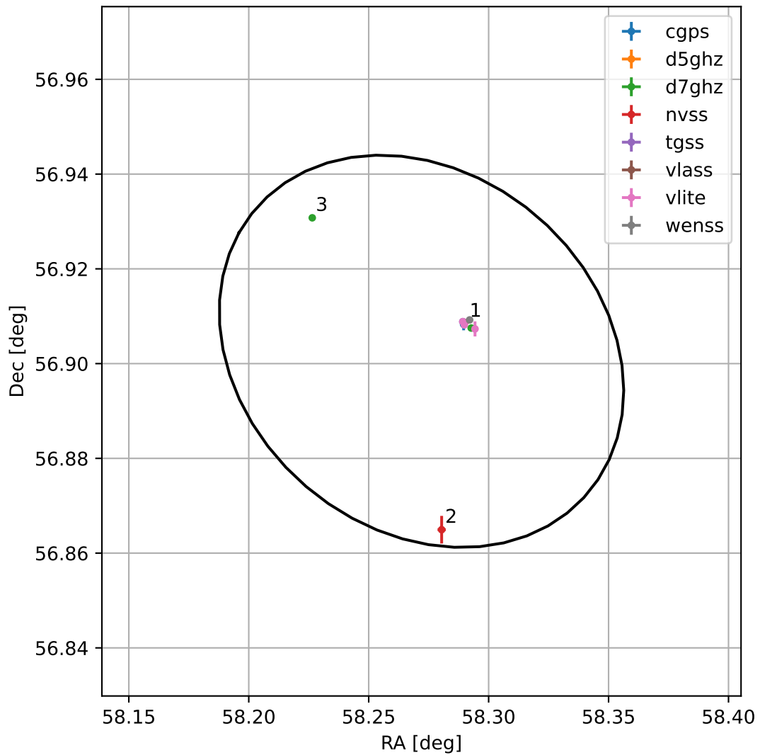
4FGL J0353.0+5654
