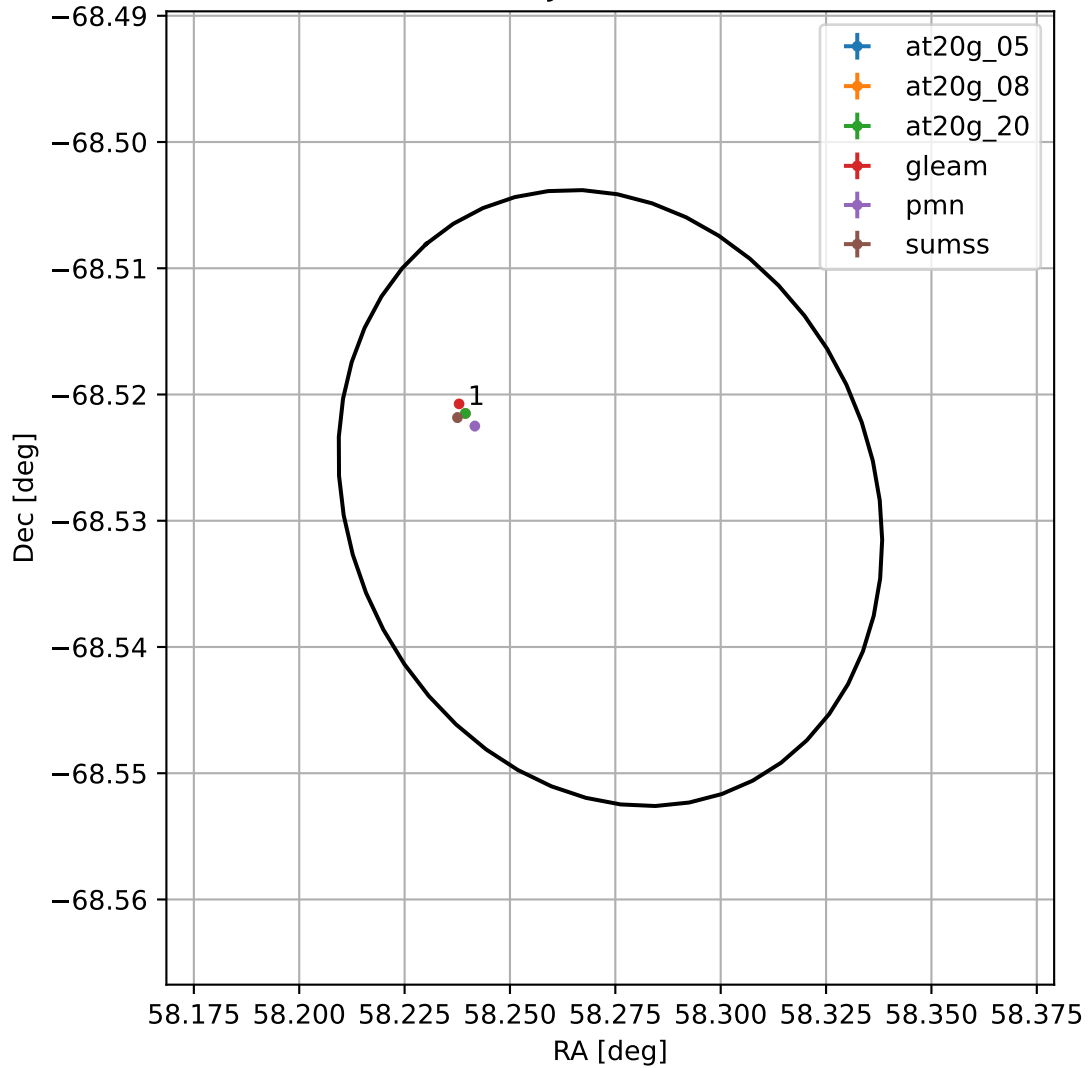
4FGL J0353.0-6831
