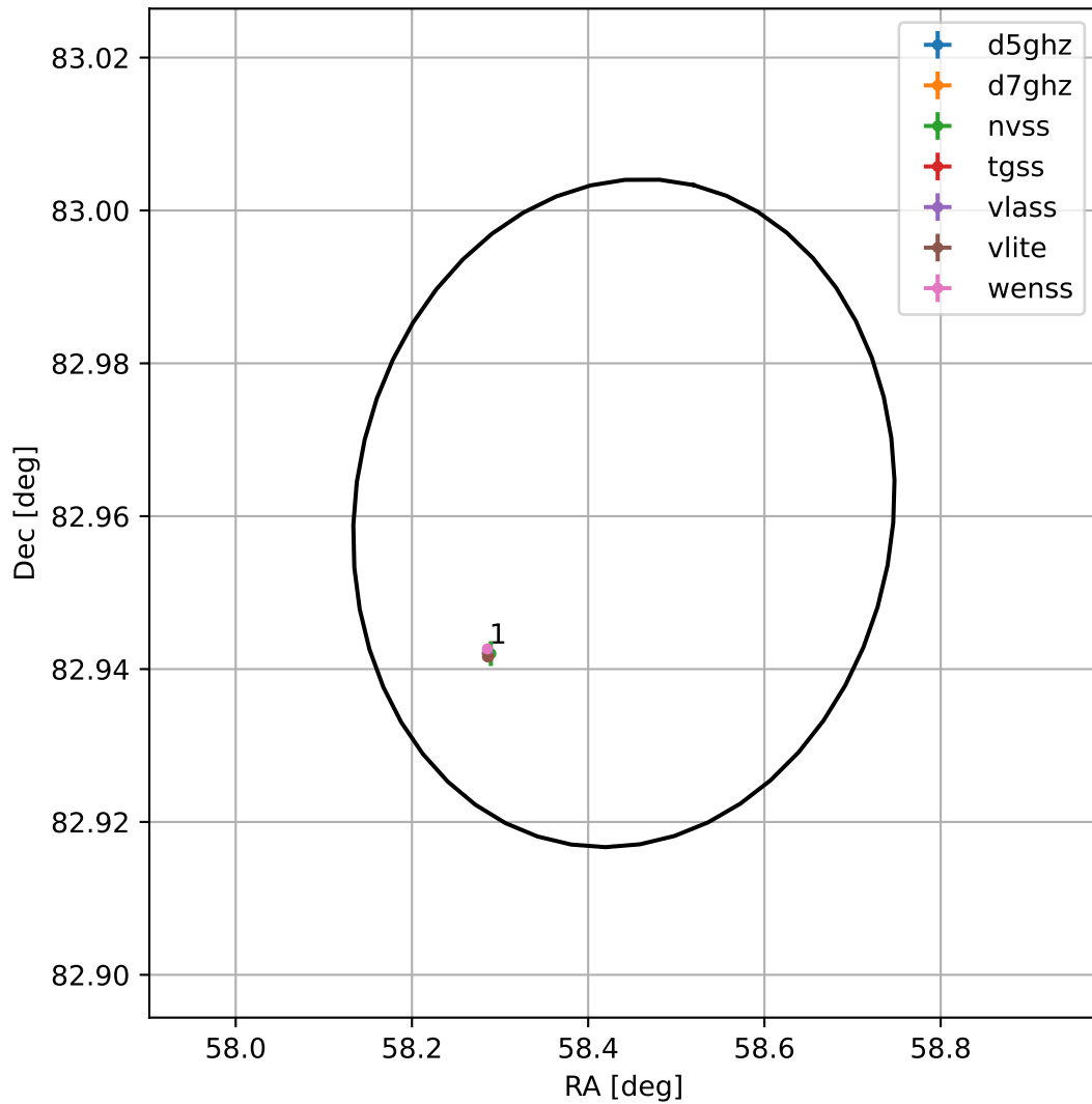
4FGL J0353.7+8257
