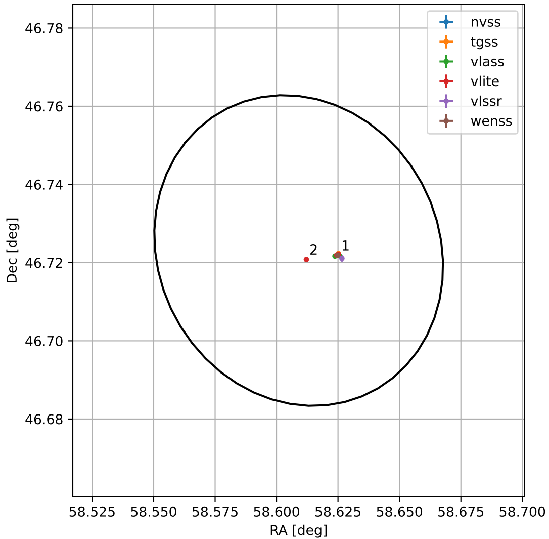
4FGL J0354.4+4643
