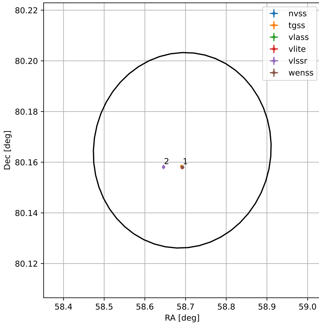
4FGL J0354.7+8009
