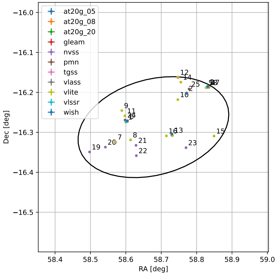
4FGL J0354.7-1617
