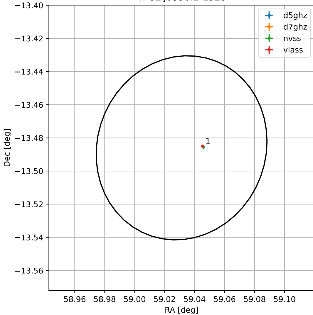
4FGL J0356.1-1329
