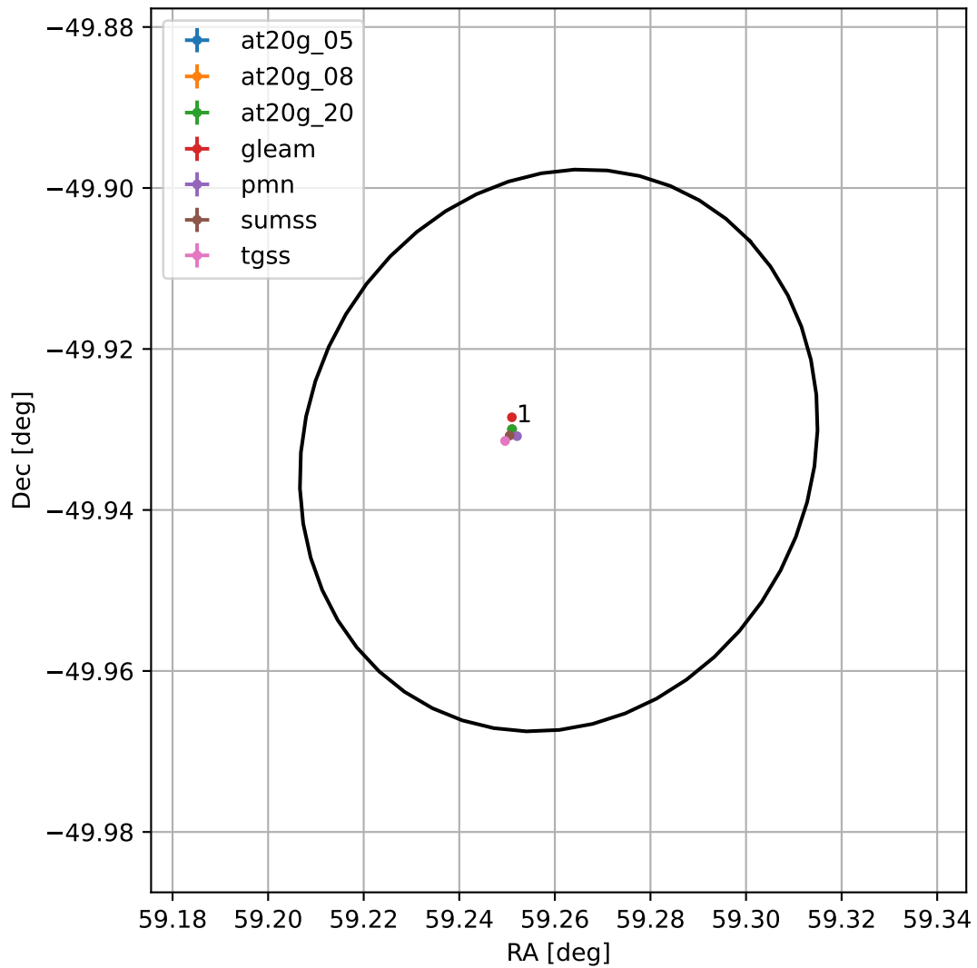
4FGL J0357.0-4955
