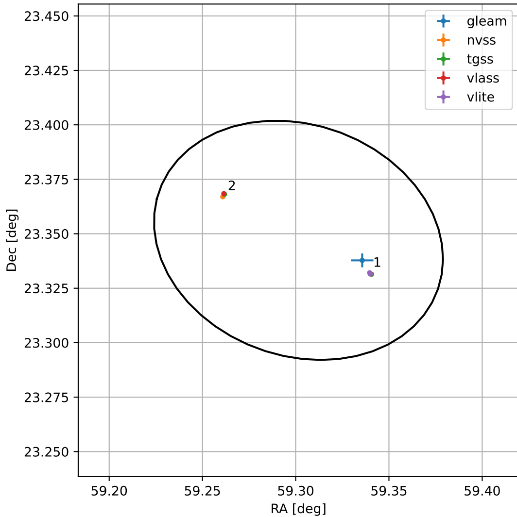
4FGL J0357.2+2320
