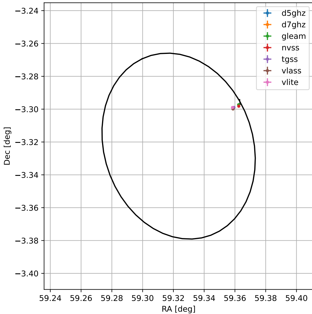
4FGL J0357.2-0319
