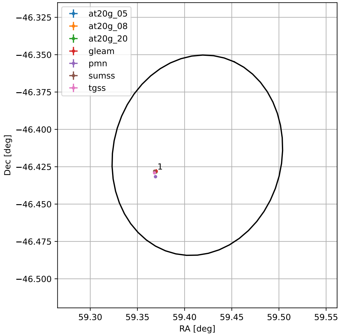
4FGL J0357.6-4625
