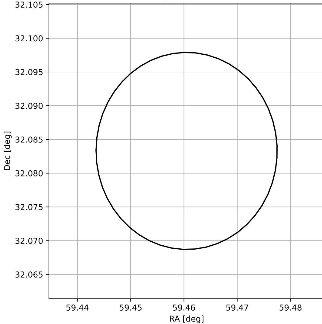
4FGL J0357.8+3204
