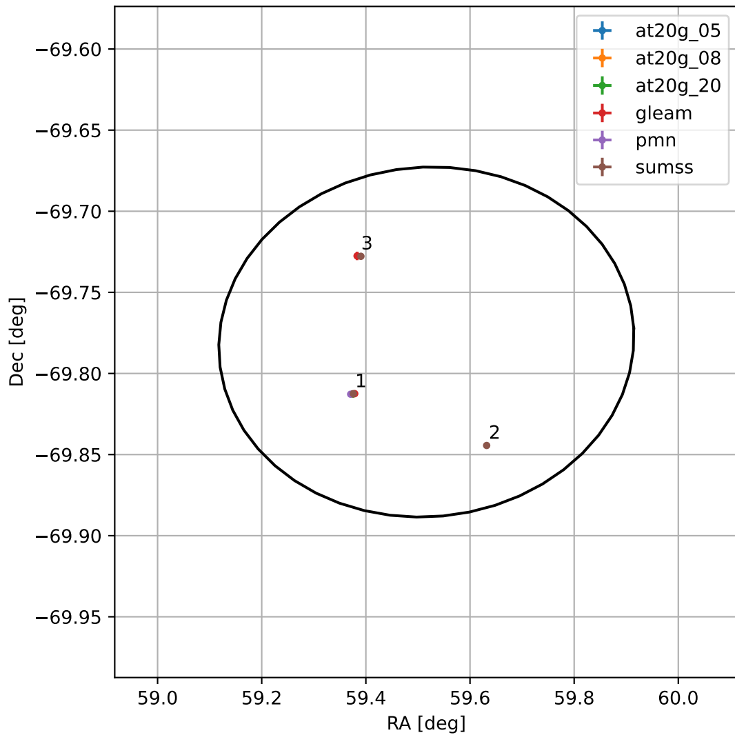
4FGL J0358.0-6946
