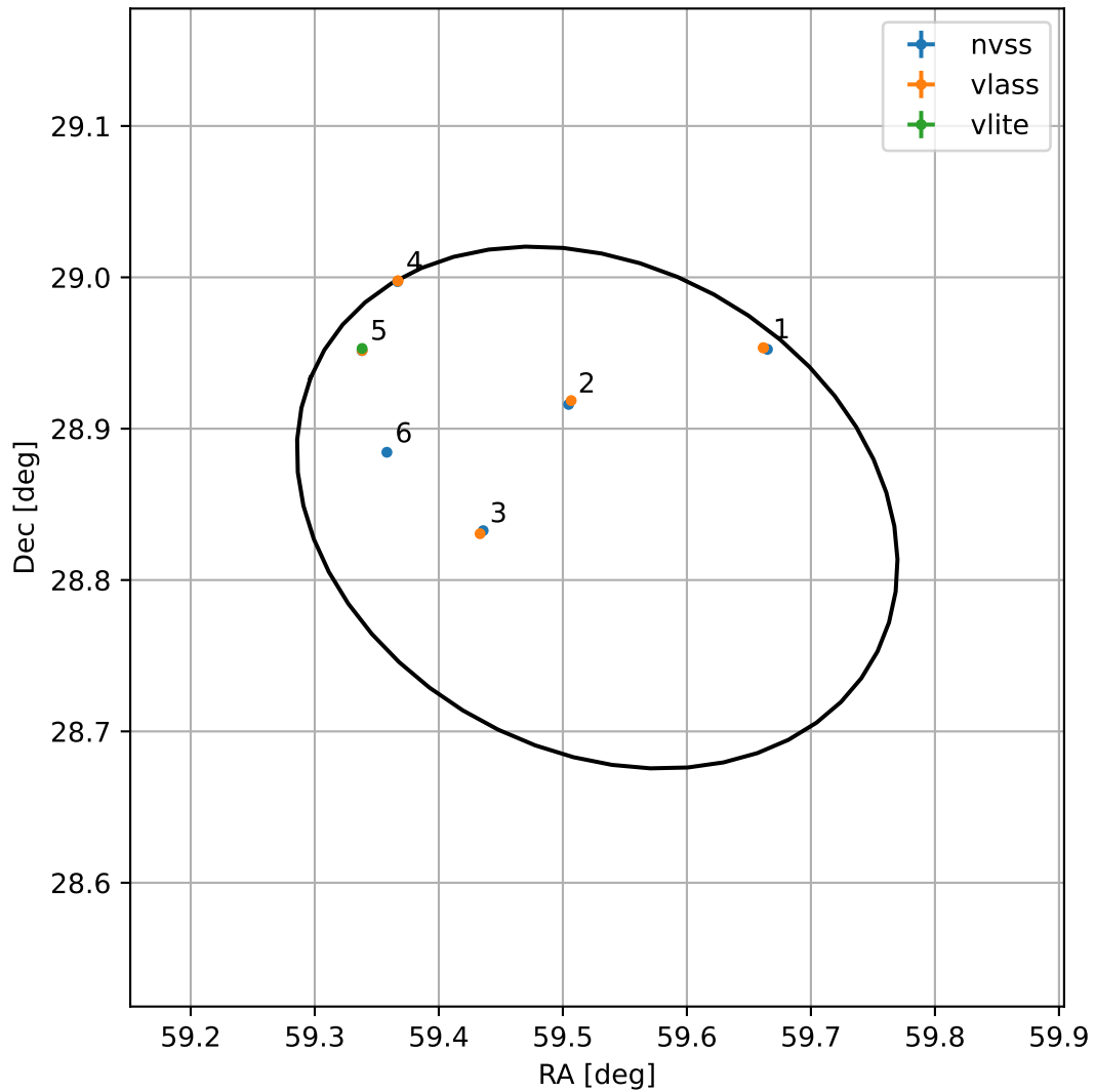
4FGL J0358.1+2850
