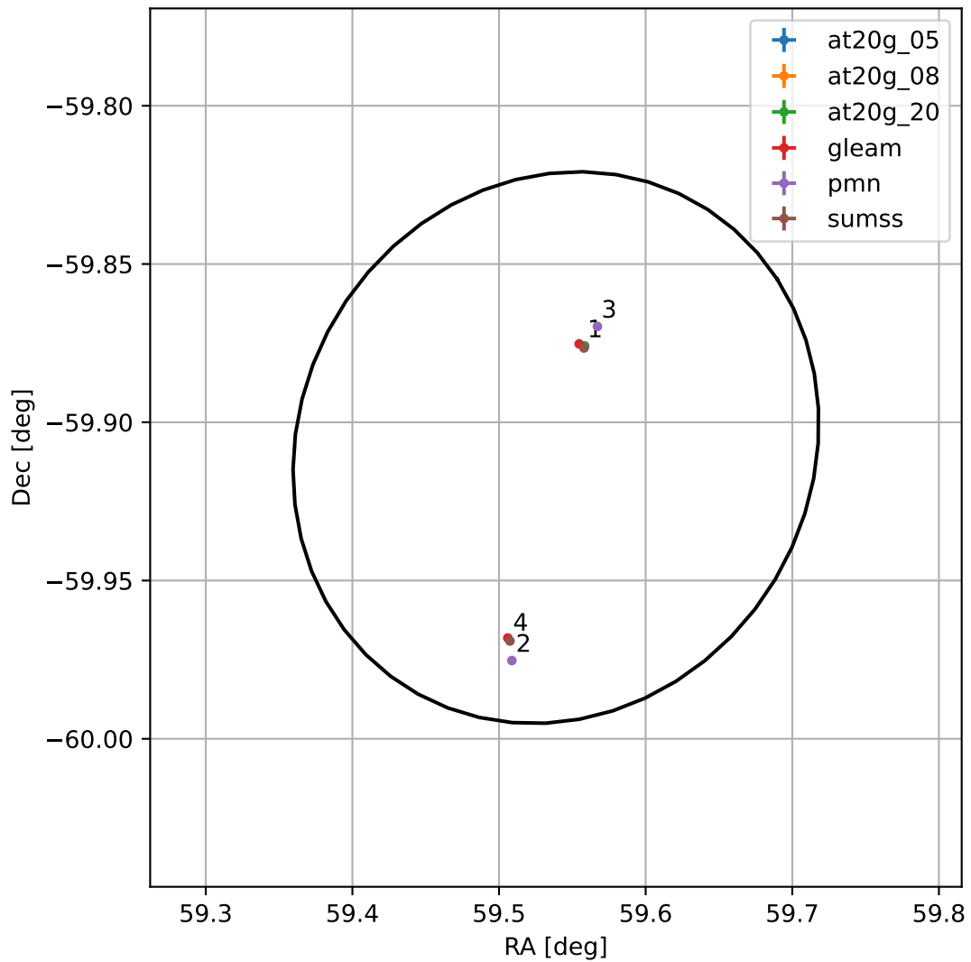
4FGL J0358.1-5954
