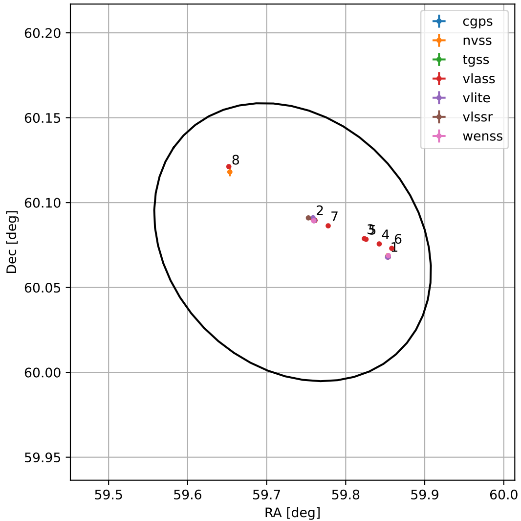
4FGL J0358.9+6004
