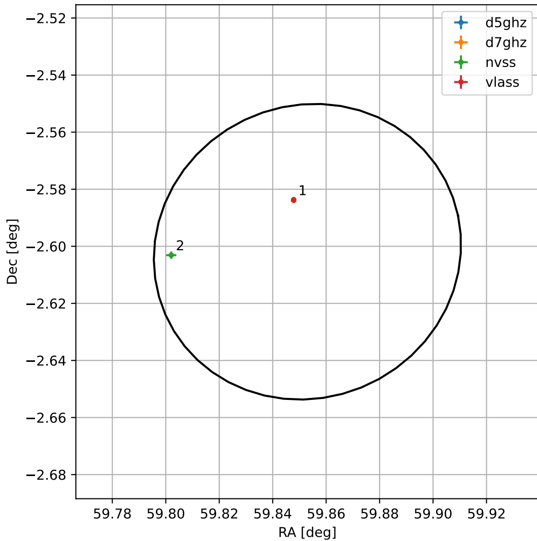
4FGL J0359.4-0236
