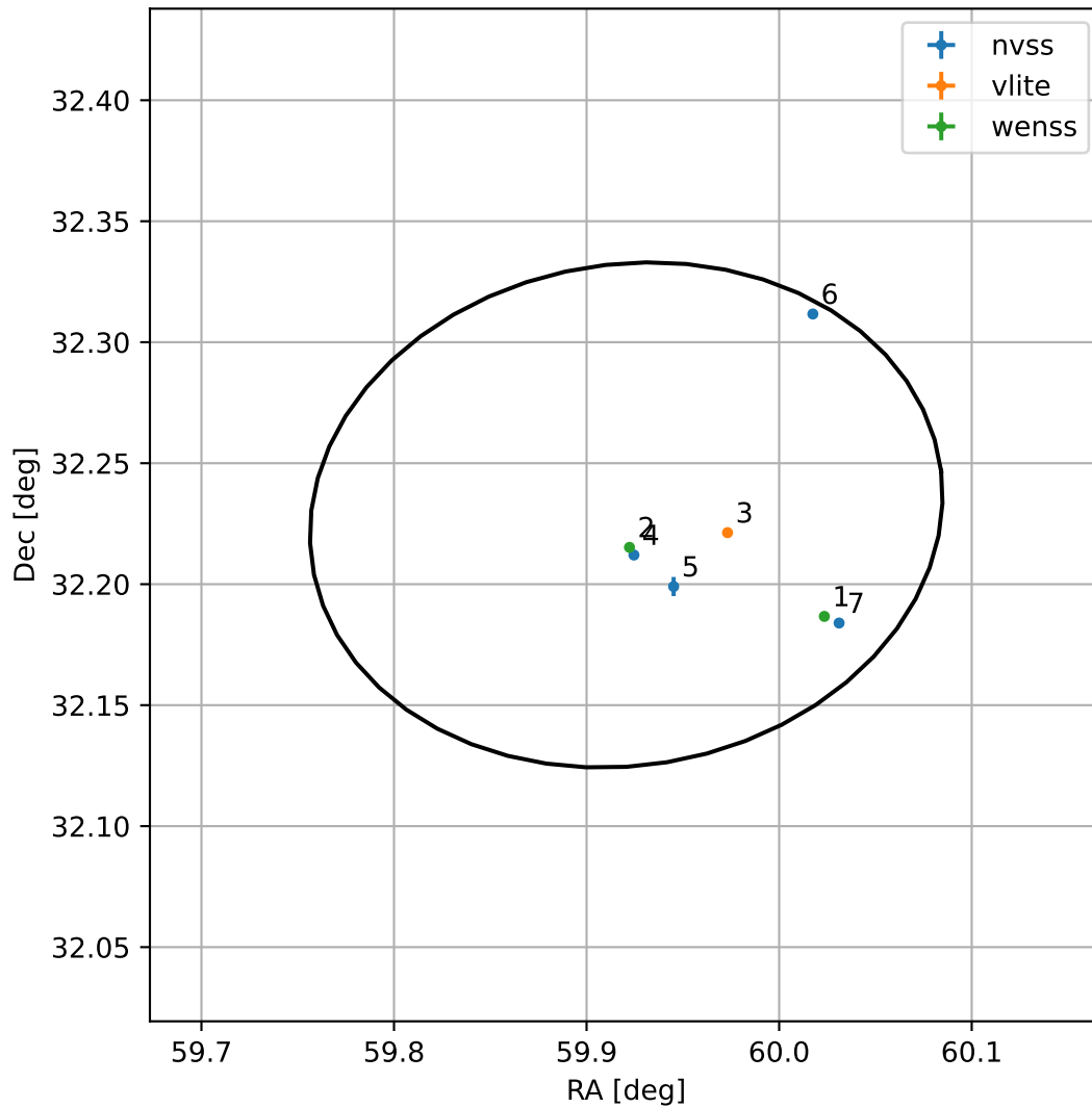
4FGL J0359.6+3213
