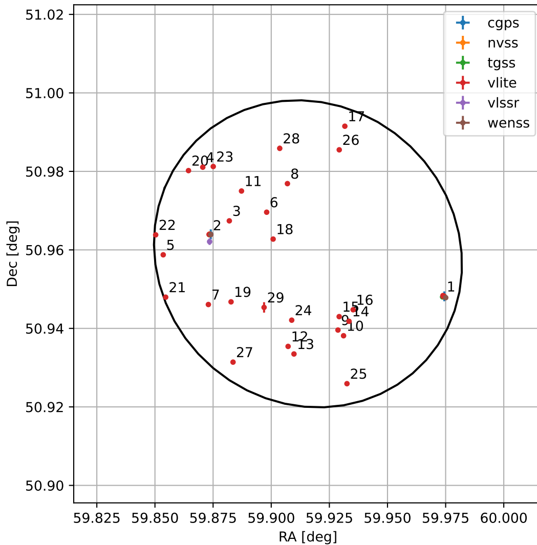
4FGL J0359.6+5057
