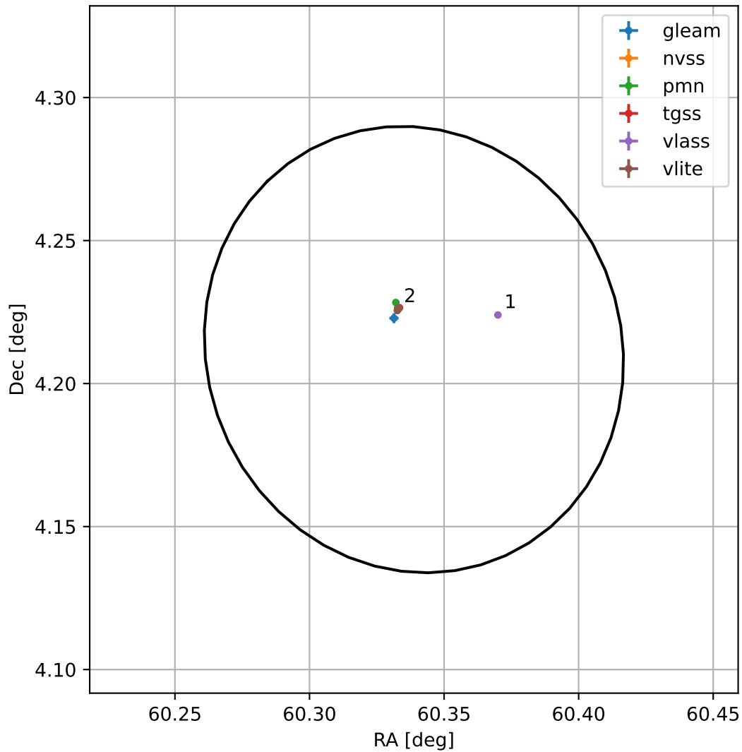
4FGL J0401.3+0412
