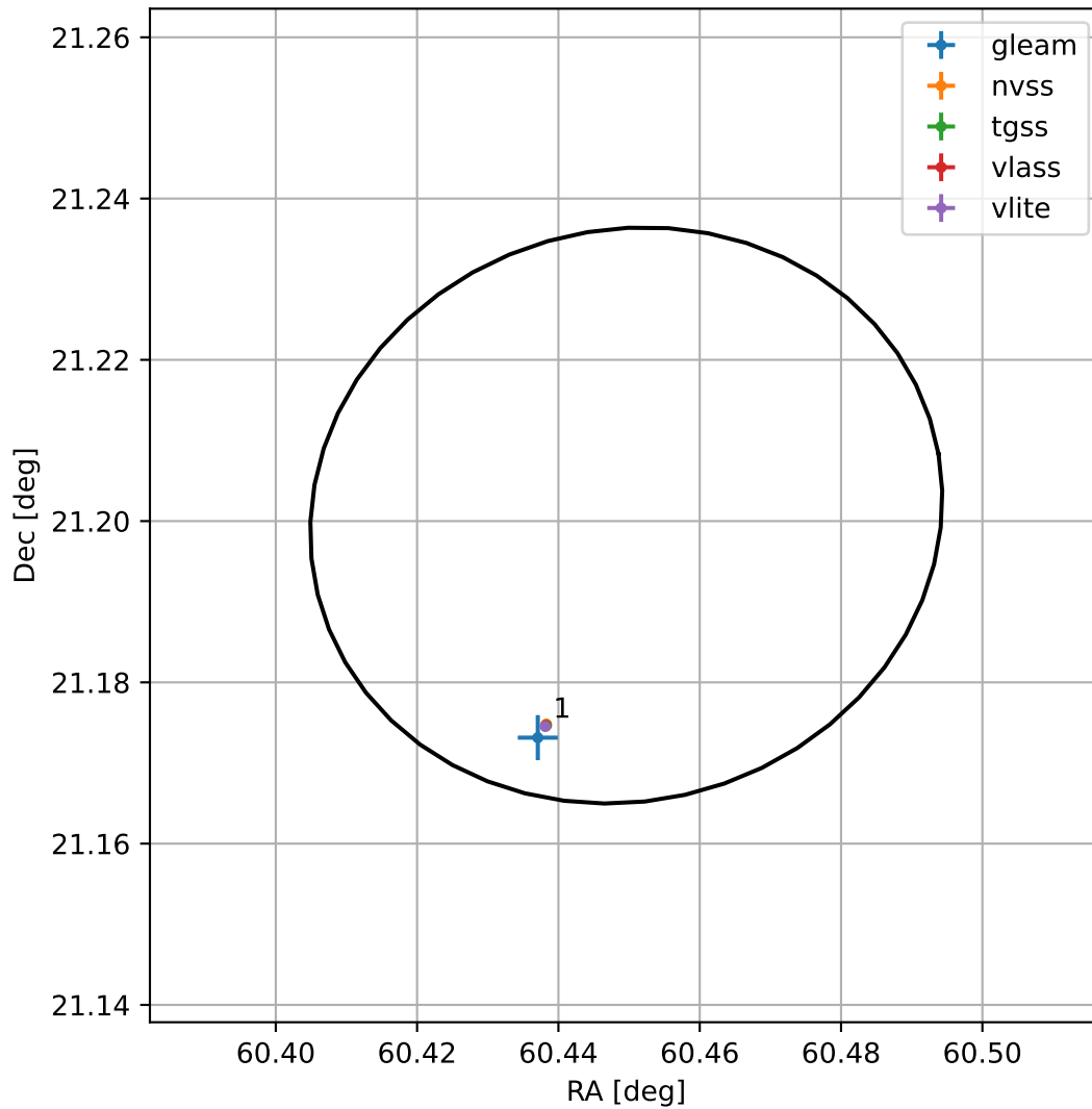
4FGL J0401.7+2112
