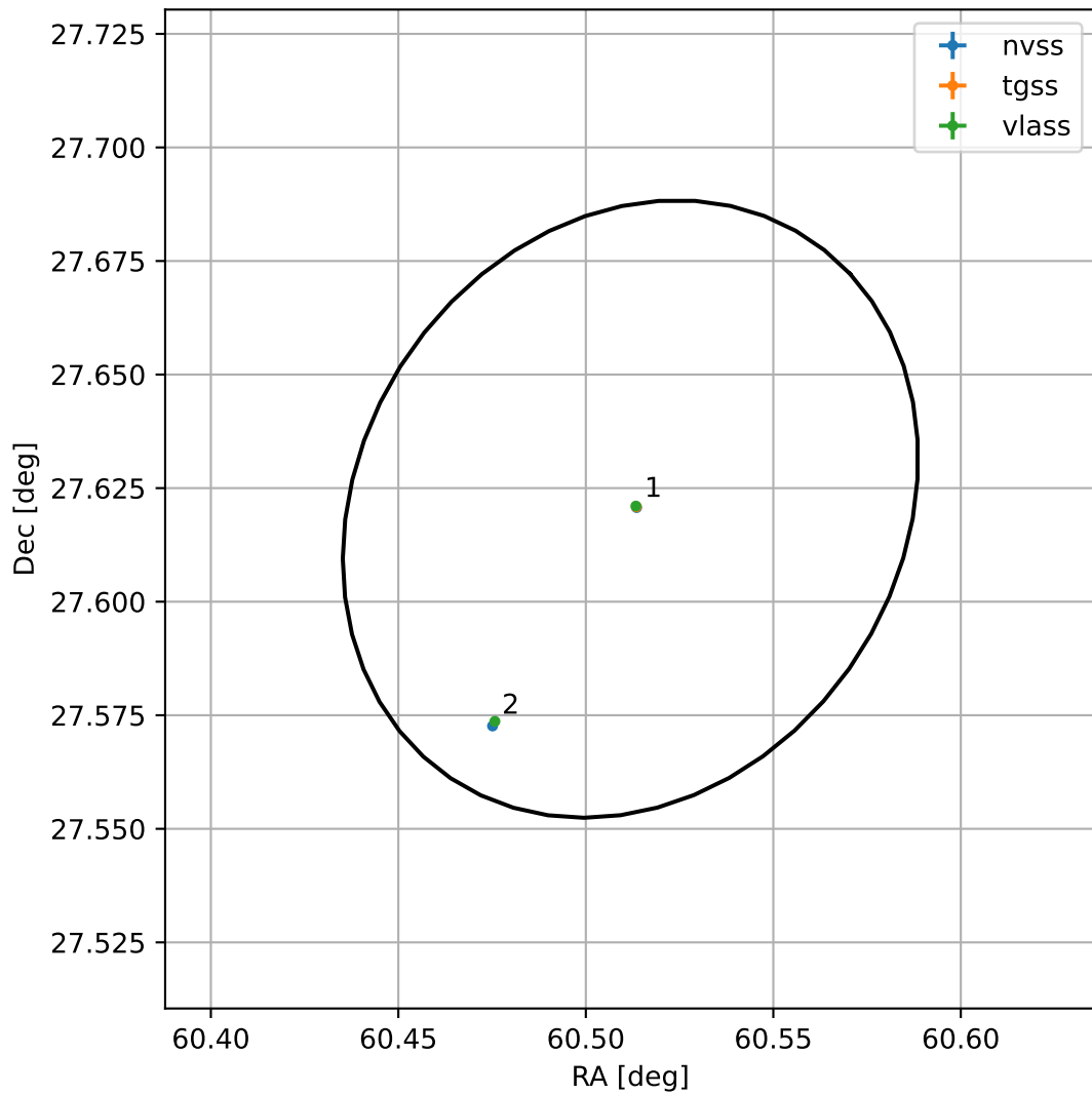
4FGL J0402.0+2737
